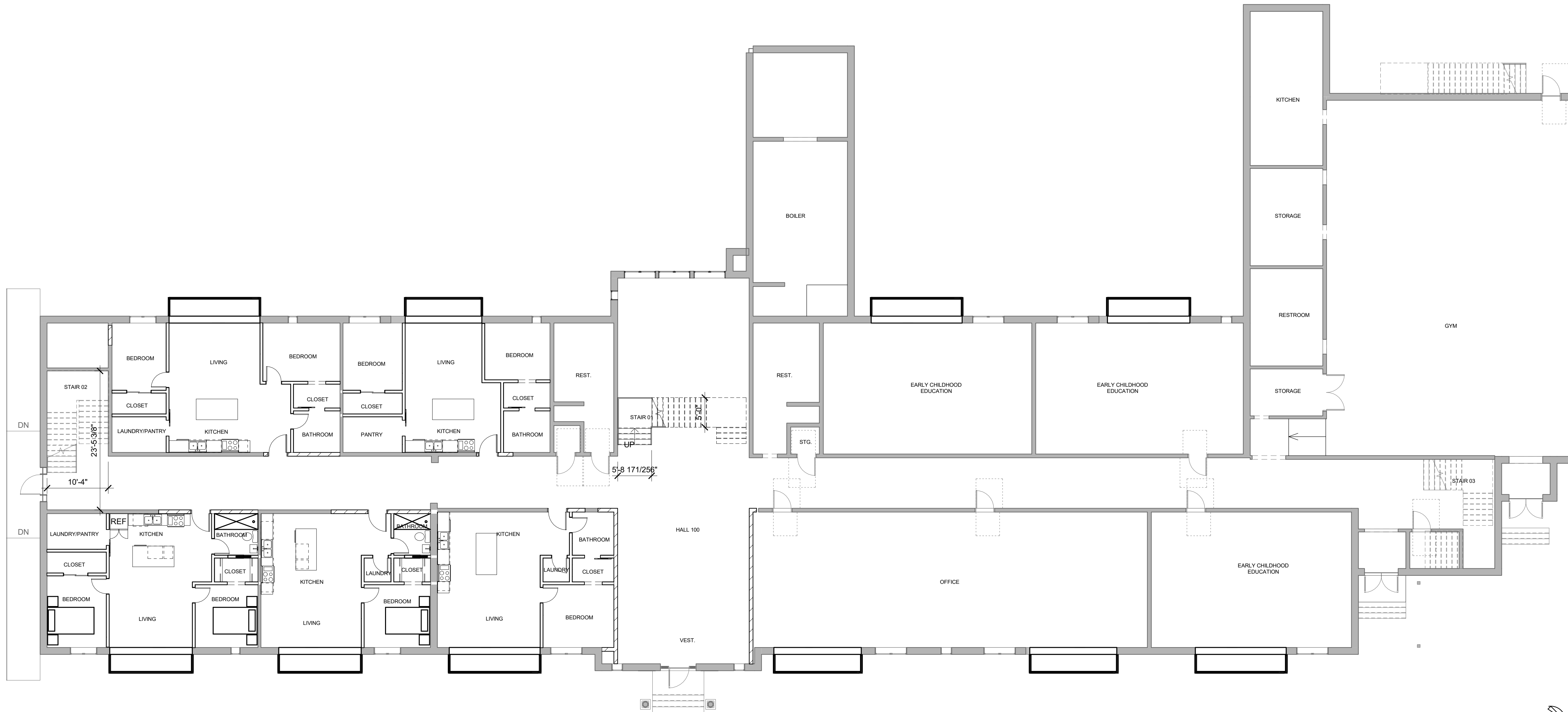
1 OVERALL FIRST FLOOR PLAN A1.03 1" = 10'-0"
